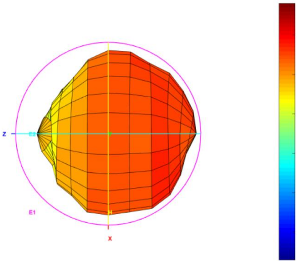
Total_3D_Left View_1.71GHz
