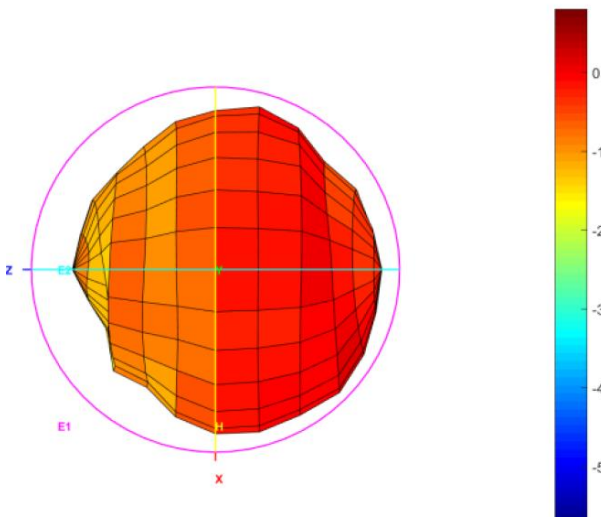
Total_3D_Top View_2.1GHz
