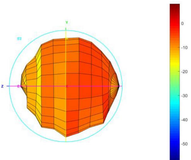
Total_3D_Left View_1.57542GHz
