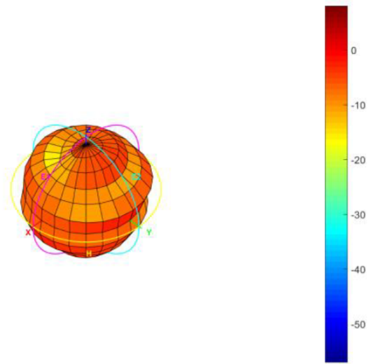
Total_3D_Side View 1_960MHz
