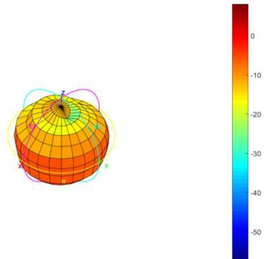
Total_3D_Side View 1_1.71GHz
