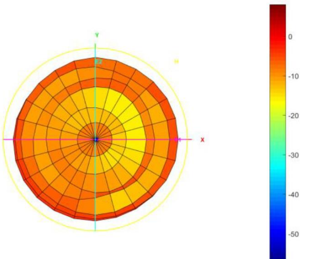
Total_3D_Front View_2.1GHz
