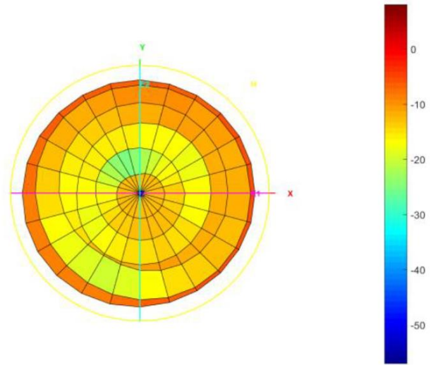
Total_3D_Side View 1_1.71GHz
