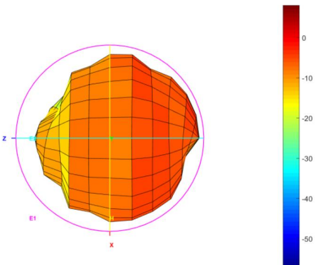
Total_3D_Top View_1.57542GHz
