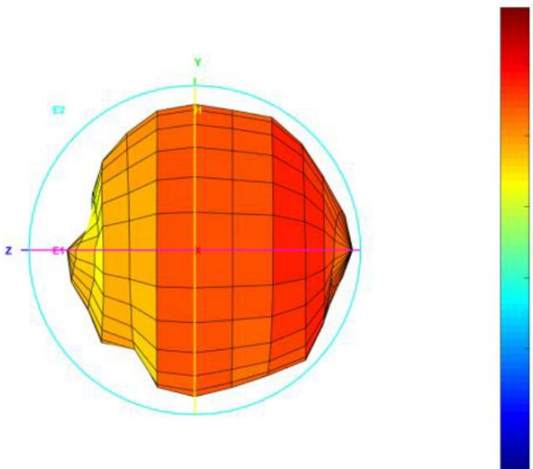
Total_3D_Left View_1.71GHz
