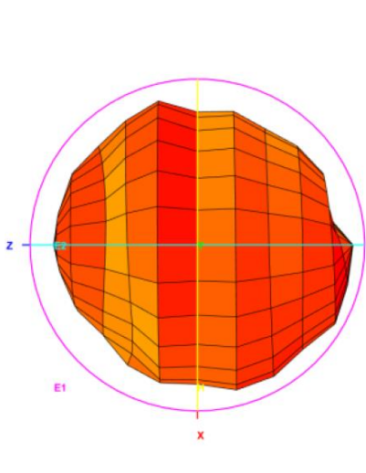
Total_3D_Top View_960MHz
