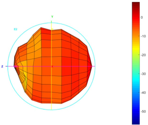
Total_3D_Left View_960MHz
