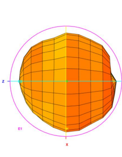
Total_3D_Top View_698MHz
