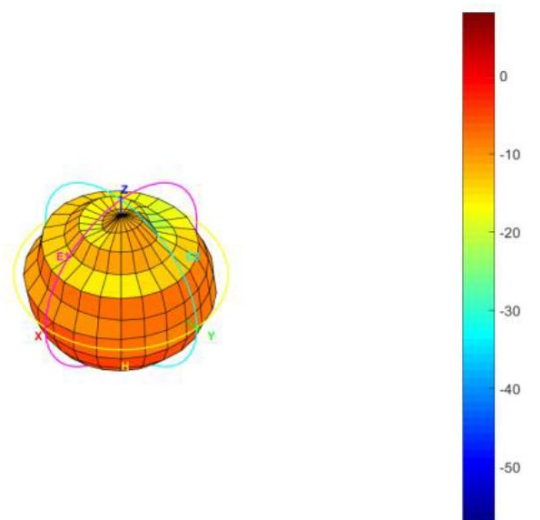
Total_3D_Side View 1_1.57542GHz
