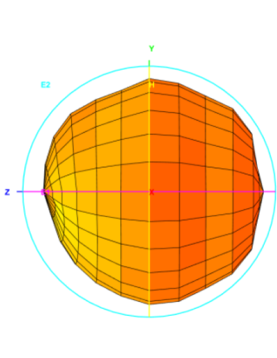
Total_3D_Left View_698MHz
