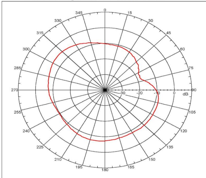
Far-field amplitude 2 100 MHz -E.nsi
